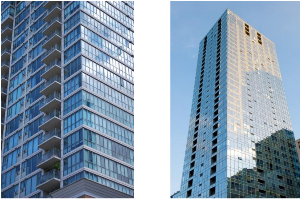
Fig.2.23 Window wall (Left) and Curtain wall (Right) assemblies occupying the majority of the vertical enclosure area of these MURBs. The air barrier system of these wall assemblies is achieved by the gaskets and sealants between the joints and interfaces of these manufactured window assemblies and interfaces to other components including slab edges.
