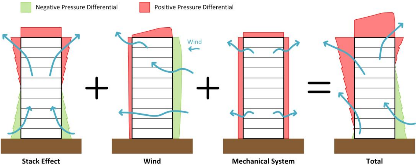
Fig.2.11 Cumulative Effect of Driving Forces of Air Movement on a tall MURB
