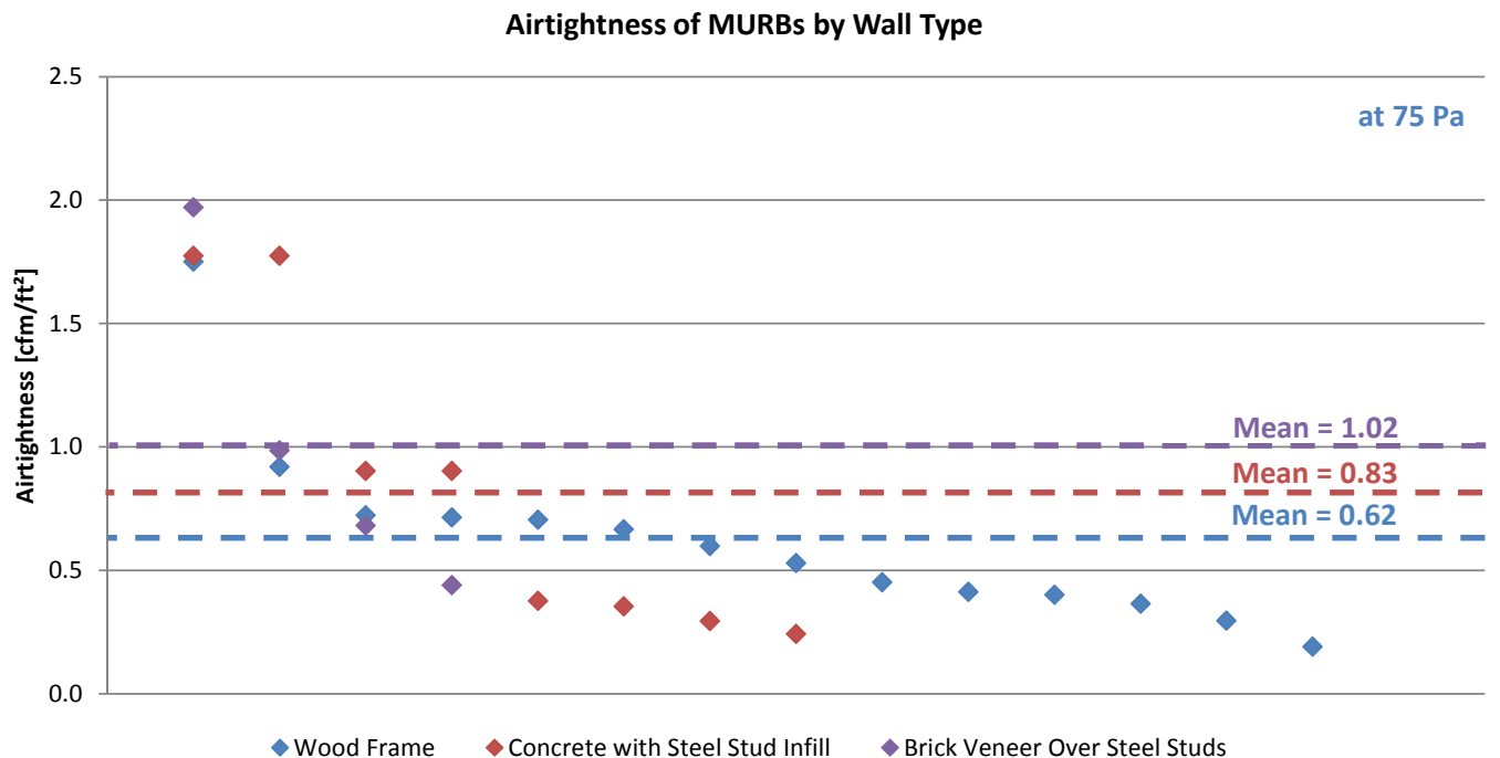
Fig.7.9 Airtightness of MURBs by Wall Type
