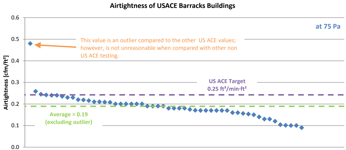
Fig.7.13 USACE Barracks Buildings Airtightness
