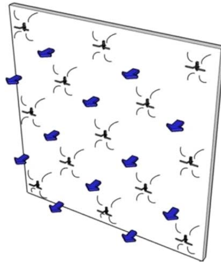
Fig.2.16 Sealed Sheathing Membrane Air Barrier Approach with Brick Ties. A limitation of the sealed sheathing membrane approach is the potential for the air barrier membrane (and WRB) to tear or become damaged around brick-tie penetrations. Solutions include SAM reinforcement over the sheathing membrane at the fastener locations or use of self-adhered and liquid membranes.
