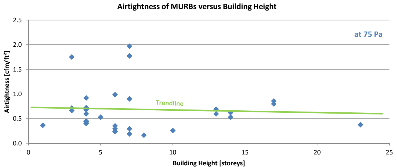
Fig.7.8 MURB Airtightness versus Building Height
