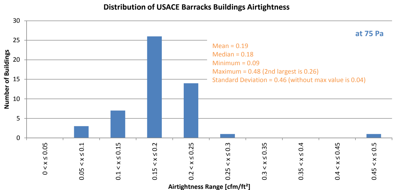
Fig.7.14 Distribution of USACE Barracks Buildings Airtightness
