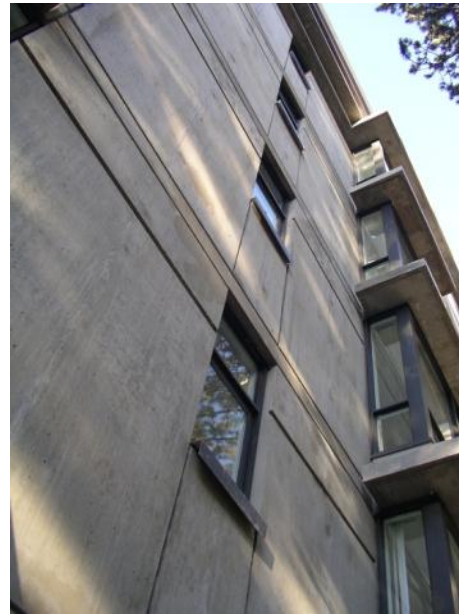
Fig.2.22 Mass Concrete Walls. Concrete and joint sealants perform the air barrier function. The proper control of cracks and joints also required for water penetration control will lead to airtight assemblies.
