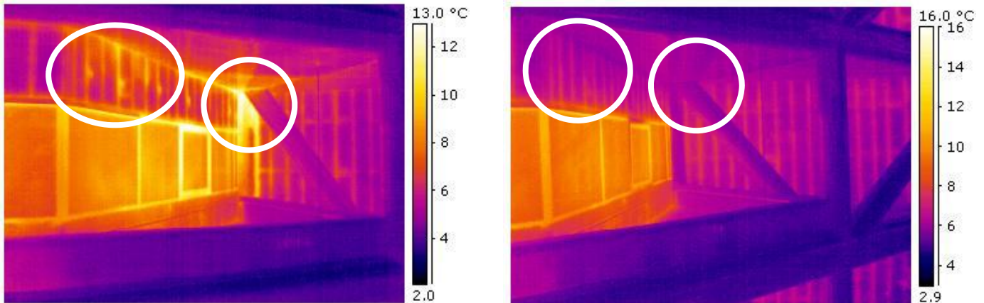
Fig.5.4 Infrared Images of MURBs from Exterior Showing Air Leakage at Operable Windows and Defects in Air Barrier Continuity
