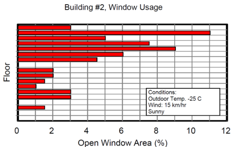
Fig.2.26 Window Usage in a 18-storey MURB in Winnipeg during -25^{\circ}\text{C} Wintertime Conditions (Proskiw and Phillips, An Examination of Air Pressure and Air Movement Patterns in Multi-Unit Residential Buildings 2006)
