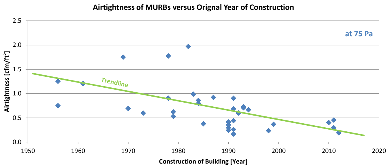
Fig.7.6 Airtightness versus Original Year of Construction
