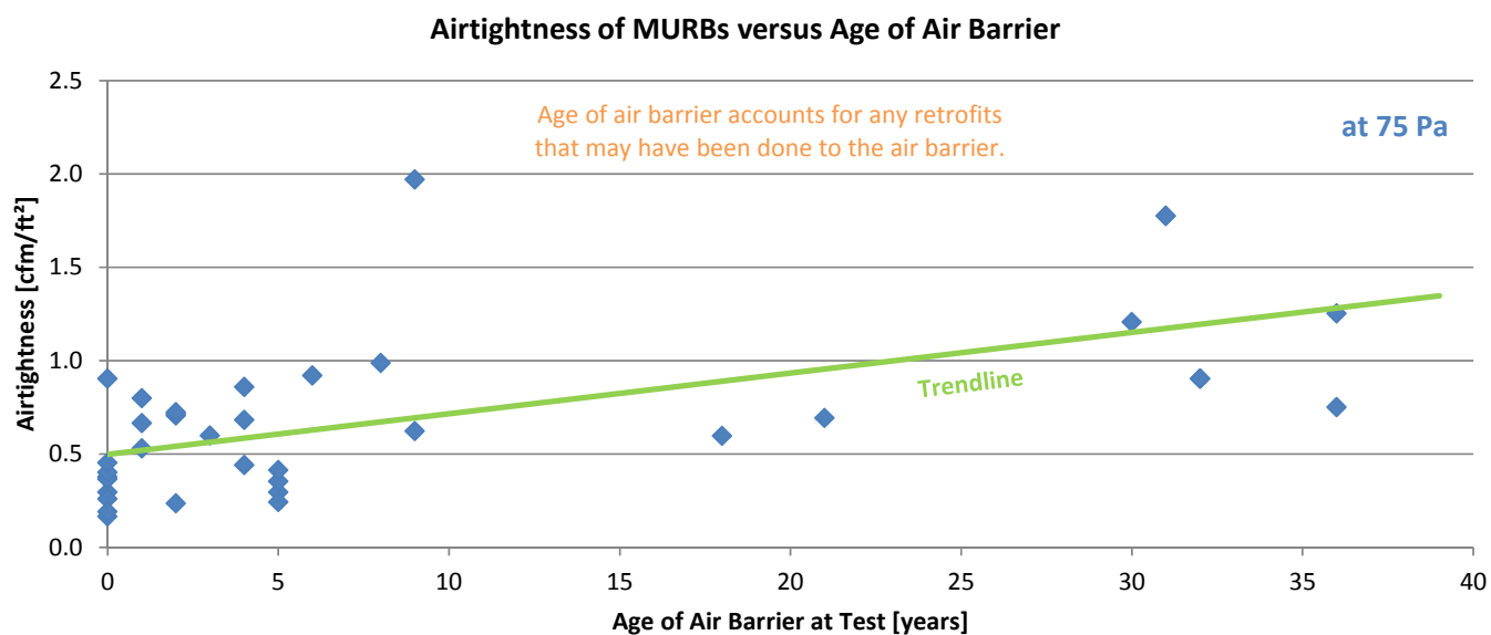
Fig.7.7 MURB Airtightness versus Age of the Air Barrier
