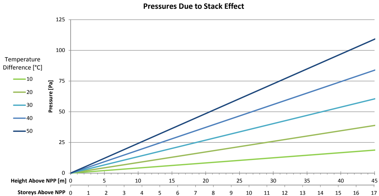
Fig.2.7 Pressure Differences Developed Due to Stack Effect in a High-rise Building (up to 90m, ~34 stories)
