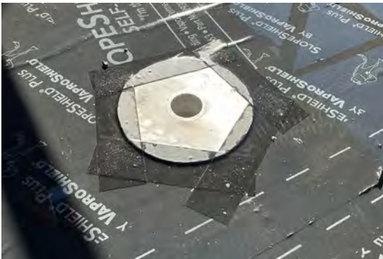
Figure 78 Drain port stripped in with tape/self-adhered membrane.
