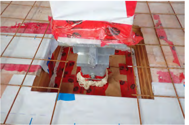
Figure 57 A temporary column detail that could collect water and does not adequately protect the end grain.
