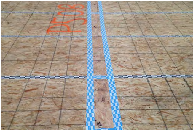
c) Vapor-impermeable tape installed at sheathing joints.
