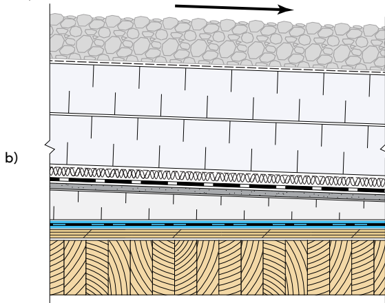
Figure 15 Protected membrane roof assembly with a) sloped mass timber panel, and b) tapered rigid insulation to create slope. The assembly layer that could potentially be utilized as the construction phase moisture protection is highlighted in blue.
