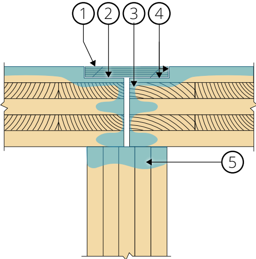
Figure 68 Moisture content reading taken at area of membrane damage.
