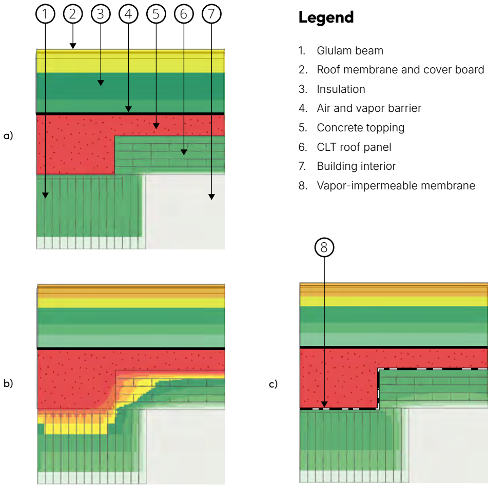
Figure 23 Two-dimensional hygrothermal model of TCC roof assembly at a column-to-panel interface where the moisture level is visualized from red (wet) to green (dry) to light green (very dry). The conditions shown are a) initial conditions immediately after a concrete pour, b) moisture migration into the wood beam and column after 12 months if no moisture protection was provided between the mass timber and concrete topping, and c) the mass timber elements maintained in a dry condition when a vapor-impermeable membrane is installed on the top and edge surfaces of the mass timber.
