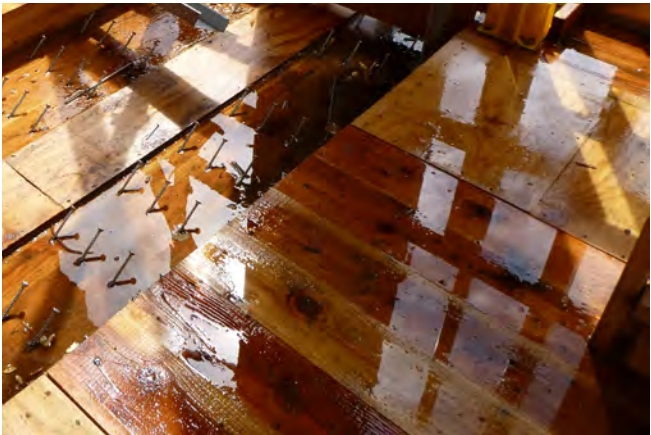
a) Moisture ponding on and absorbing into a timber-concrete composite (TCC) floor panel before the concrete is scheduled.
