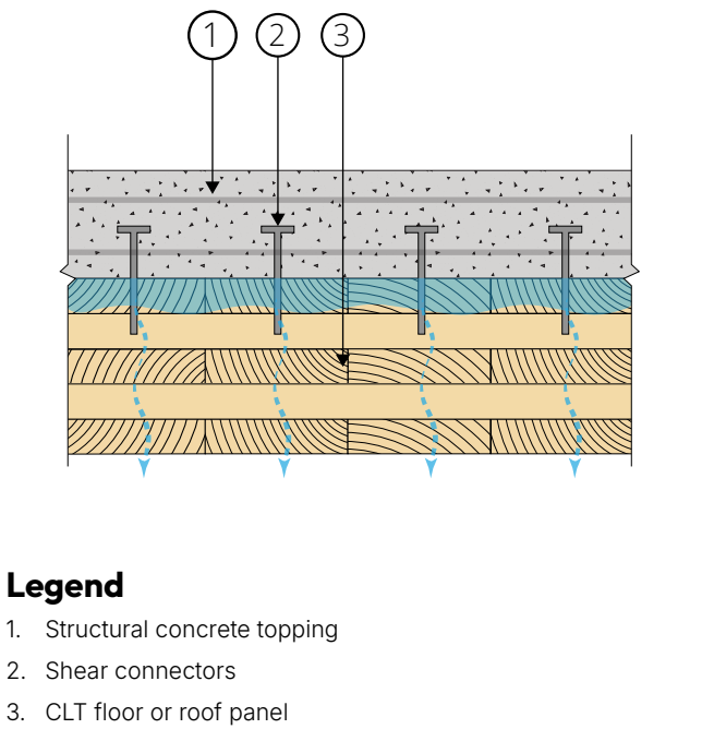
Figure 21 Timber-concrete composite assembly. The installation of a temporary membrane in addition to the topping essentially eliminates drying of the topside of the mass timber panel; therefore, the mass timber needs to be confirmed dry (i.e., less than 16% moisture content) prior to the placement of a topping.
