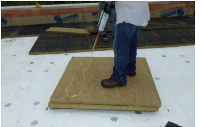
Figure 18 A roof assembly with a fastened-adhered hybrid attachment system. The first layer of insulation is mechanically fastened, but subsequent insulation layers are adhered. The fasteners are installed through the membrane, which acts as the construction phase moisture protection and the permanent air and vapor barrier.
